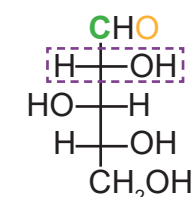
D-Xylose
