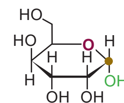
\alpha -D-Glucose
